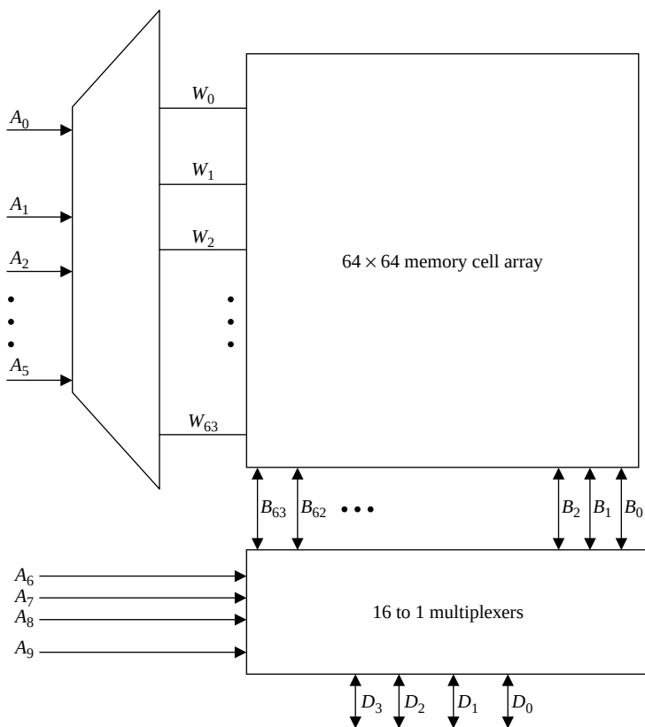
Figure 7.4 Efficient internal organization of a 1K×4 memory chip
