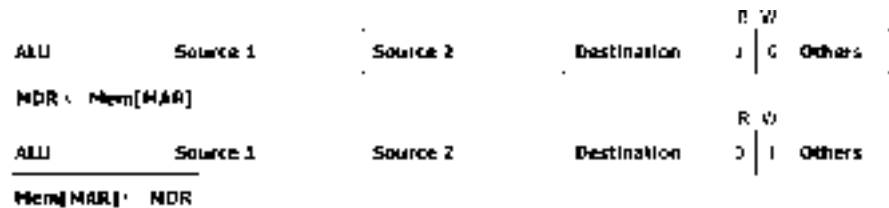
Figure 5.16 Microinstructions for memory read and write
