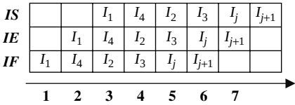
Figure 9.10 Instruction reordering
