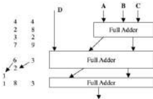
Figure 9.20 Carry-save addition
