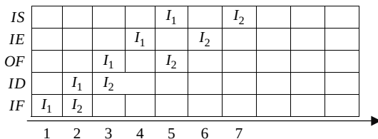
Figure 9.14 Hardware forwarding
