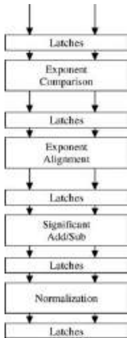
Figure 9.19 A schematic for a pipeline FP adder
