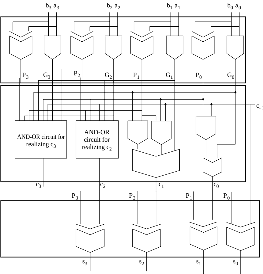
Figure 4.5 A 4-bit CLA adder structure
