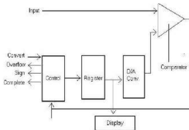
Figure 16.5: Successive Approximation
