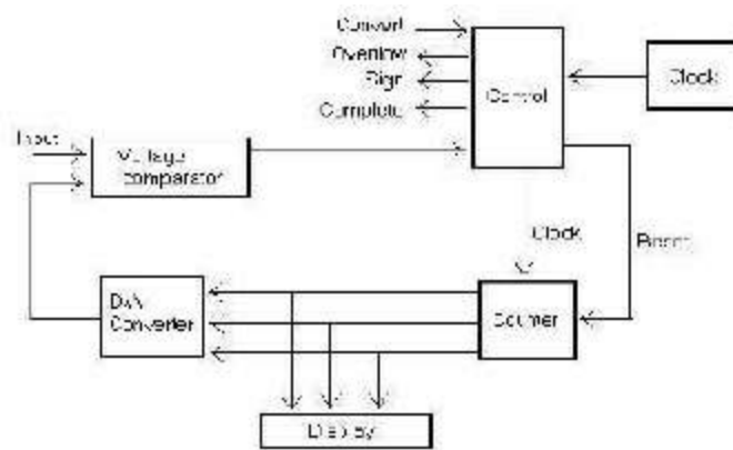
Figure 16.4: Ramp Conversion
